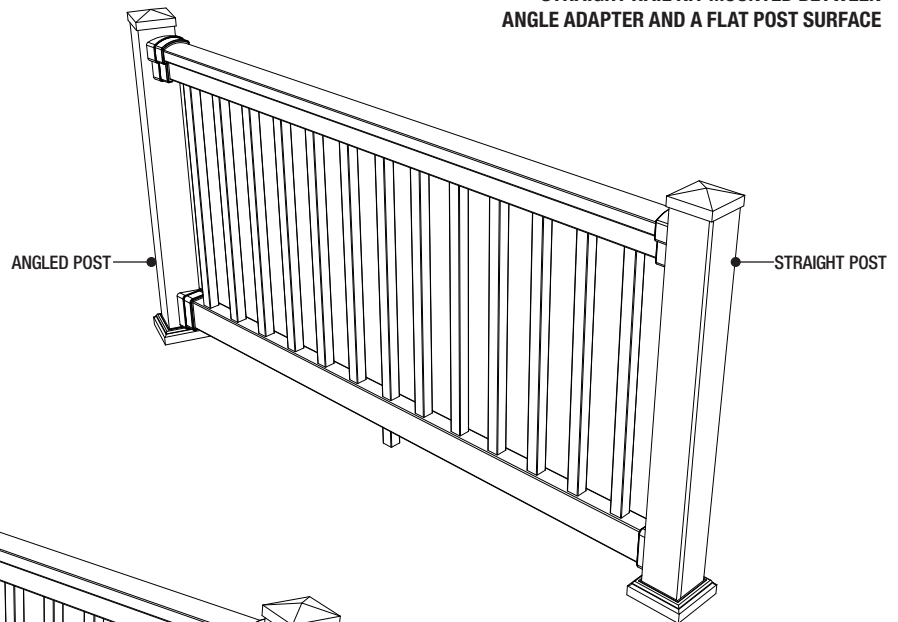
STRAIGHT RAIL KIT MOUNTED BETWEEN ANGLE ADAPTER AND A FLAT POST SURFACE
