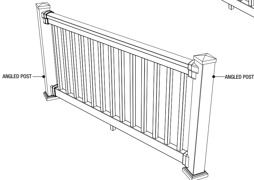
STRAIGHT RAIL KIT MOUNTED BETWEEN ANGLE ADAPTERS
