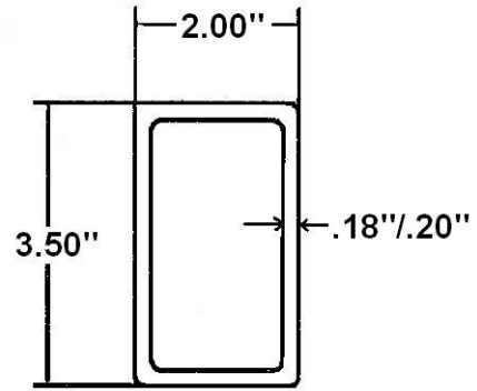
Bottom Rail (1)
