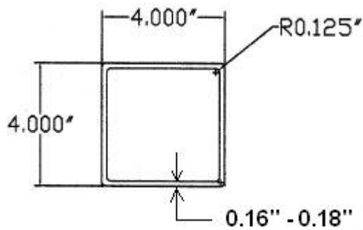
Figure 3 TAM-RAIL® 4x4 Post Sleeve Cross Section
