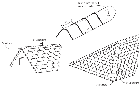
Diagram: C LAMARITE Site-Made Hip & Ridge
