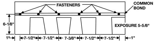
MANSARD AND HIGH WIND WARRANTY FASTENING PATTERN
