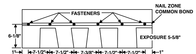
MANSARD AND HIGH WIND WARRANTY FASTENING PATTERN
